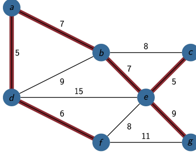
Figure 2: Illustration of Spanning Tree Constraint from Example 4
